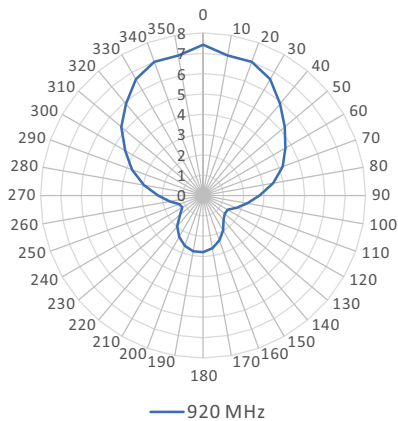
Radiation Pattern
