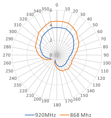
Radiation Pattern
